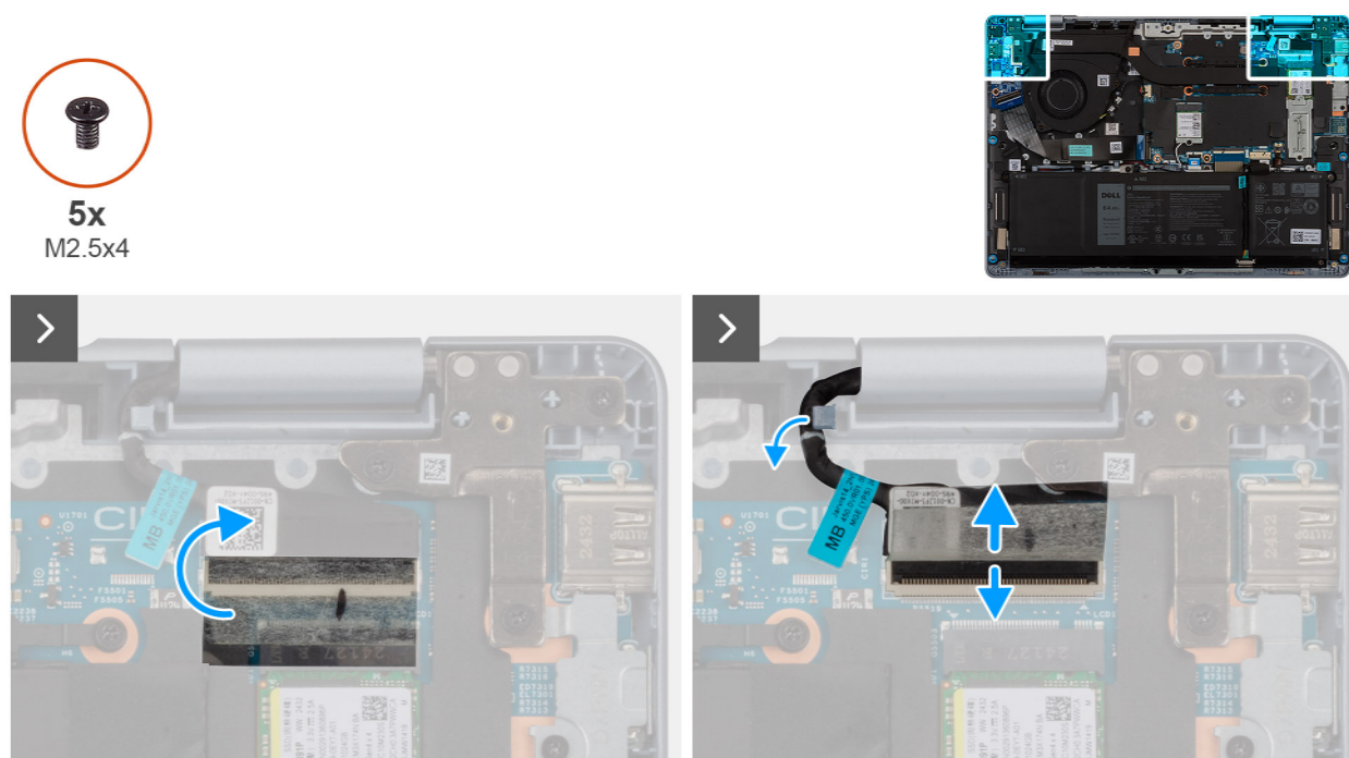
Figure 42. Disconnecting the display cable
