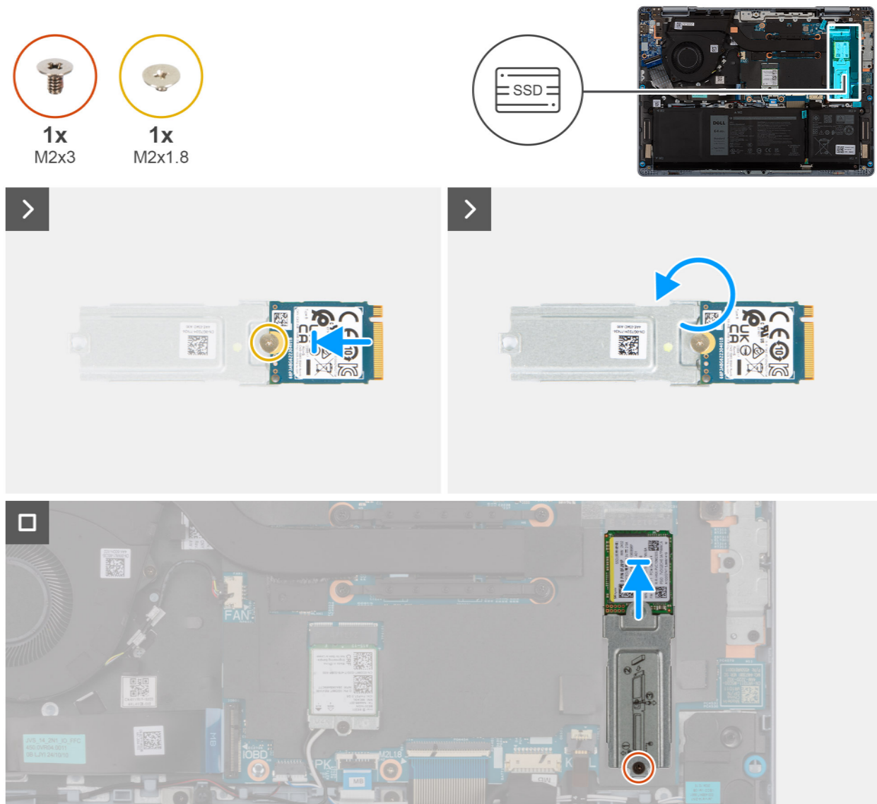
Figure 23. Installing the solid-state drive
