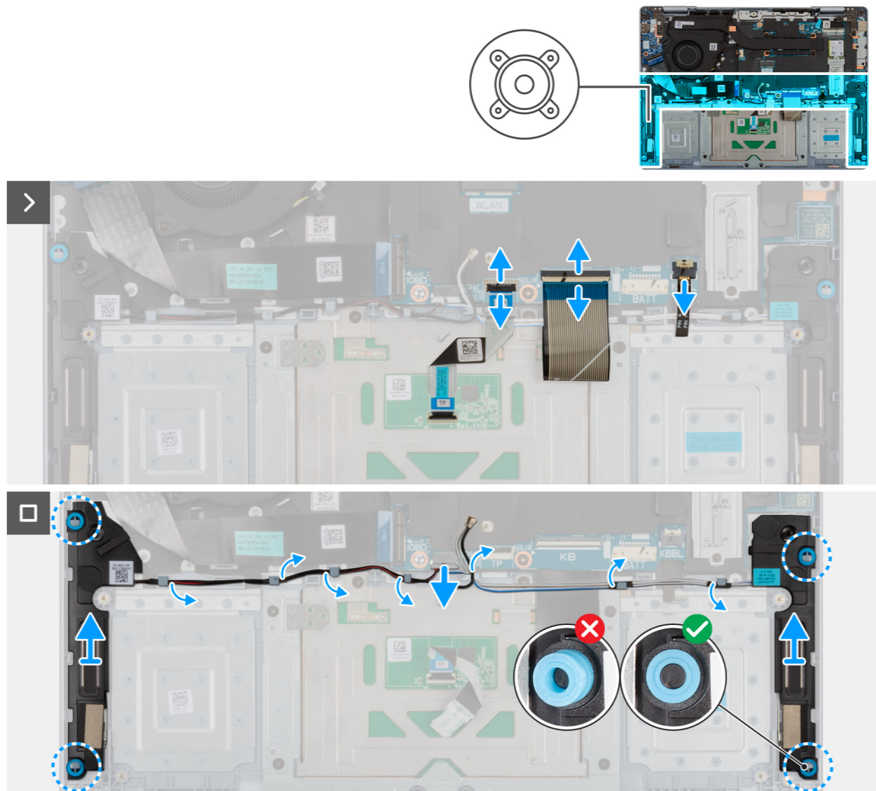
Figure 40. Removing the speakers
